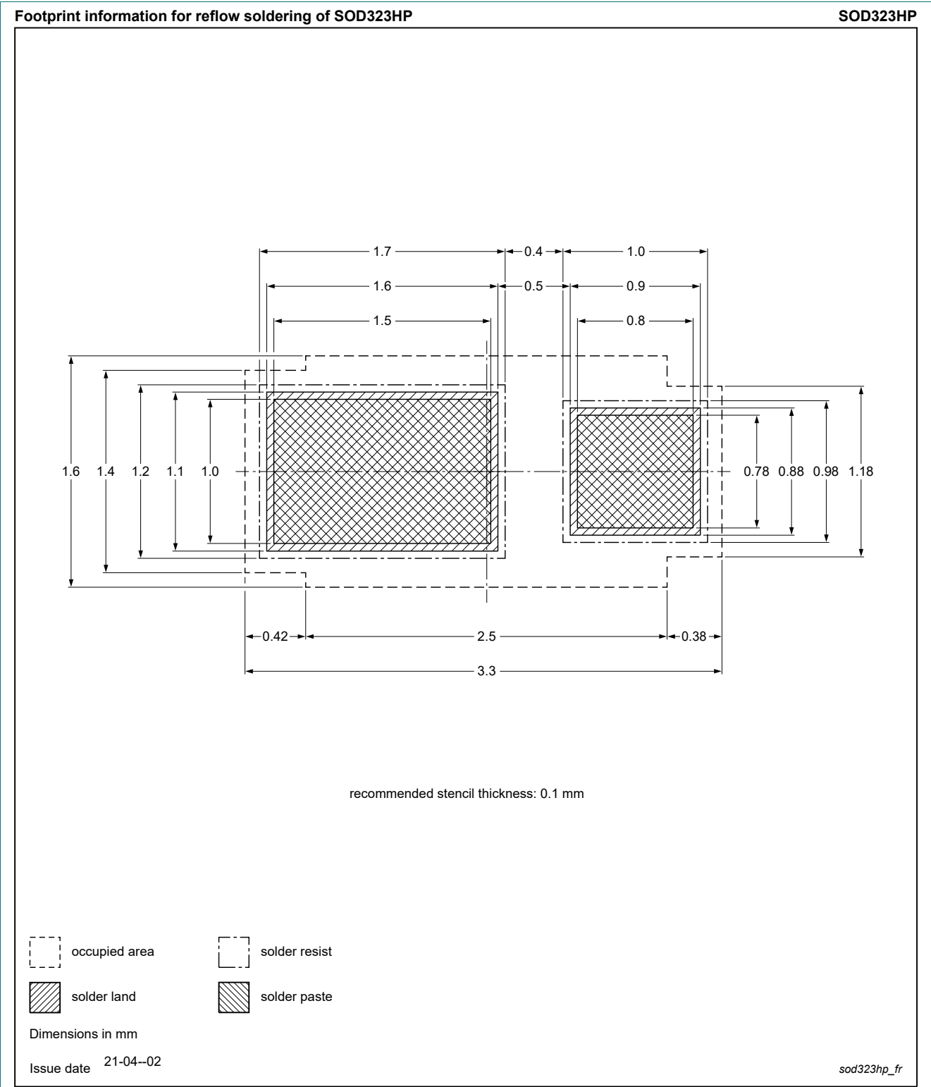
Fig. 16. Reflow soldering footprint for CFP2-HP (SOD323HP)
